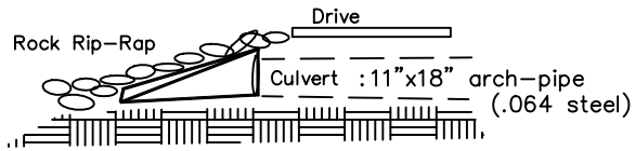
12 L5 Culvert w/ Flair End Detail N.T.S.
