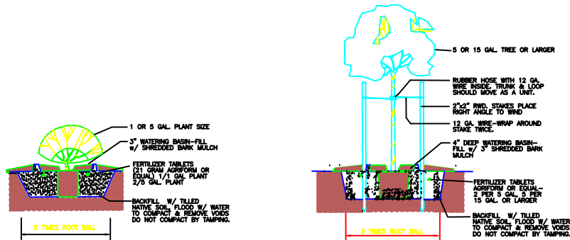
Shrub Planting Detail N.T.S.
